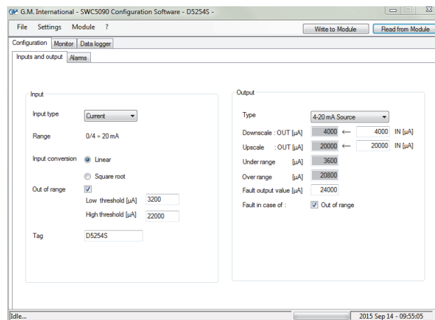
D6254S Input/Output screen
