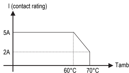
Contact Current rating vs Operating Ambient Temperature:
